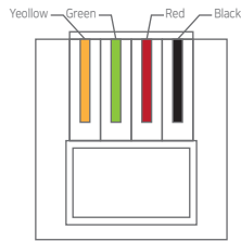
RJ-11 Terminal Wiring
